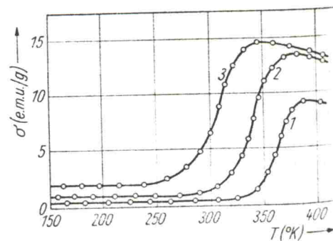
Fig. 2. Temperature dependence of magnetizations in Mn_2Ge_{0.20}Sb_{0.80} samples in magnetic fields of different strength. (1) H = 27 kOe, (2) H = 100 kOe, and (3) H = 240 kOe
