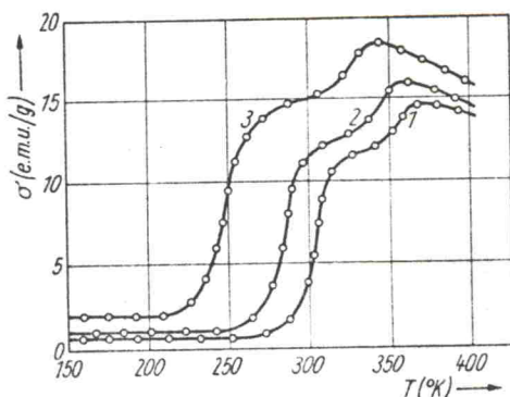
Fig. 1. Temperature dependence of the magnetization of Mn_2Ge_{0.16}Sb_{0.84} samples in magnetic fields of different strength. (1) H = 53 kOe, (2) H = 106 kOe, and (3) H = 212 kOe
